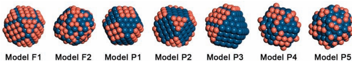
Figure 6. Structural models calculated by DFT and MD simulations for the purpose of comparing them to values extracted from fits to the XAS spectra of \text{G6-OH}(\text{Pt}_{147}@\text{Cu}_{\text{full}}) and \text{G6-OH}(\text{Pt}_{147}@\text{Cu}_{\text{partial}}) . Model F1 is the full shell model generated by the deposition of Cu atoms onto both the Pt(100) and Pt(111) facets of \text{Pt}_{147}^{\text{DFT}} as shown in Figure 3; Model F2 is a surface-alloyed structure that resulted when MD simulations were applied to structural model F1; Model P1 is the partial shell model generated by the deposition of Cu atoms onto only the Pt(100) facets of \text{Pt}_{147}^{\text{DFT}} as shown in Figure 3; Model P2 is another partial shell model in which Cu occupies only the Pt(111) facet positions; Model P3 is a partial shell model in which the Cu atoms are arranged in a Janus-like partial shell coverage; Model P4 is a partial shell model having most of the Cu atoms deposited in the Pt(100) facets and a small degree of dispersion of the Cu shell atoms to the Pt(111) facets; Model P5 is a partial shell structure created by randomly distributing Cu atoms over the entire surface.
